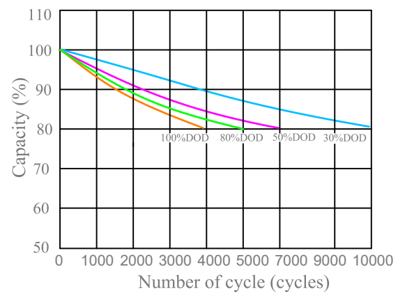
Cycle life with DOD at 25°C, 1C/1C
