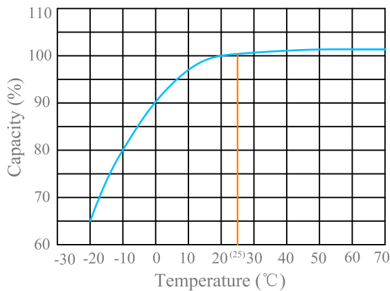
Temperature effects on capacity at 1C
